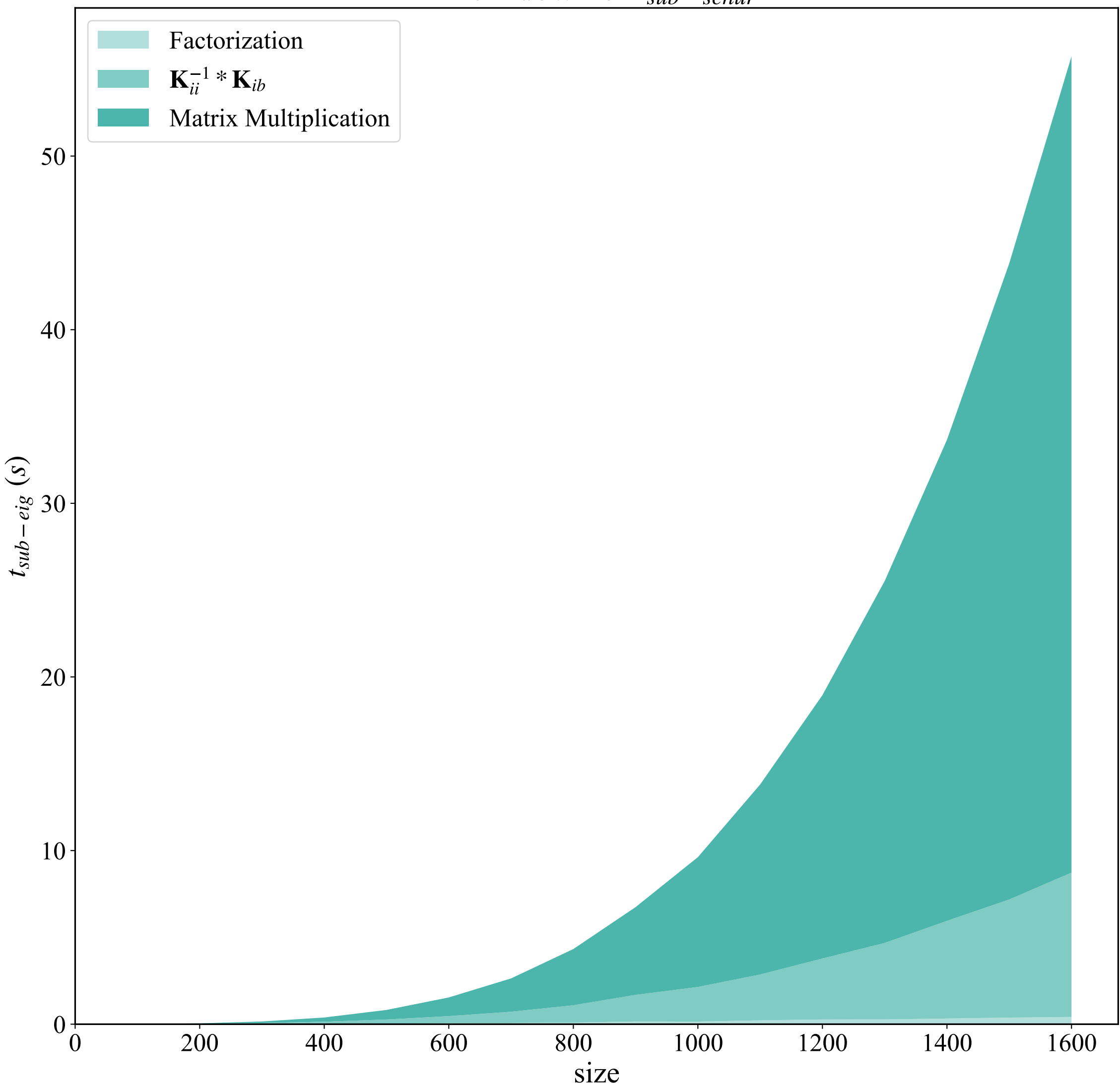
Breakdown of t_{sub-schur}
