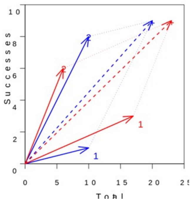
Vector interpretation
