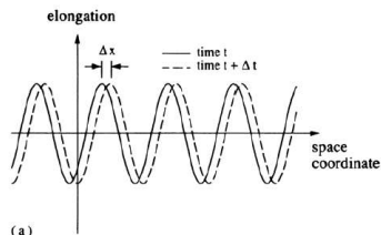
A monochromatic wave
