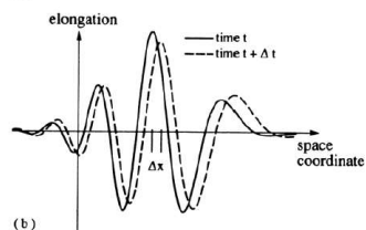
Fig. 2.1. A harmonic wave (a) and a wave packet (b) shown at two different times t and t + \Delta t to illustrate the concepts of phase and group velocity, respectively
