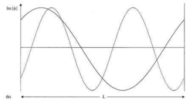
Fig. 2.3. Plane waves which have nodes at the boundaries (a) or which obey periodic boundary conditions (b)
