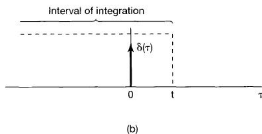
Figure 1.37 Running integral given in eq. (1.71): (a) t < 0 ; (b) t > 0 .
