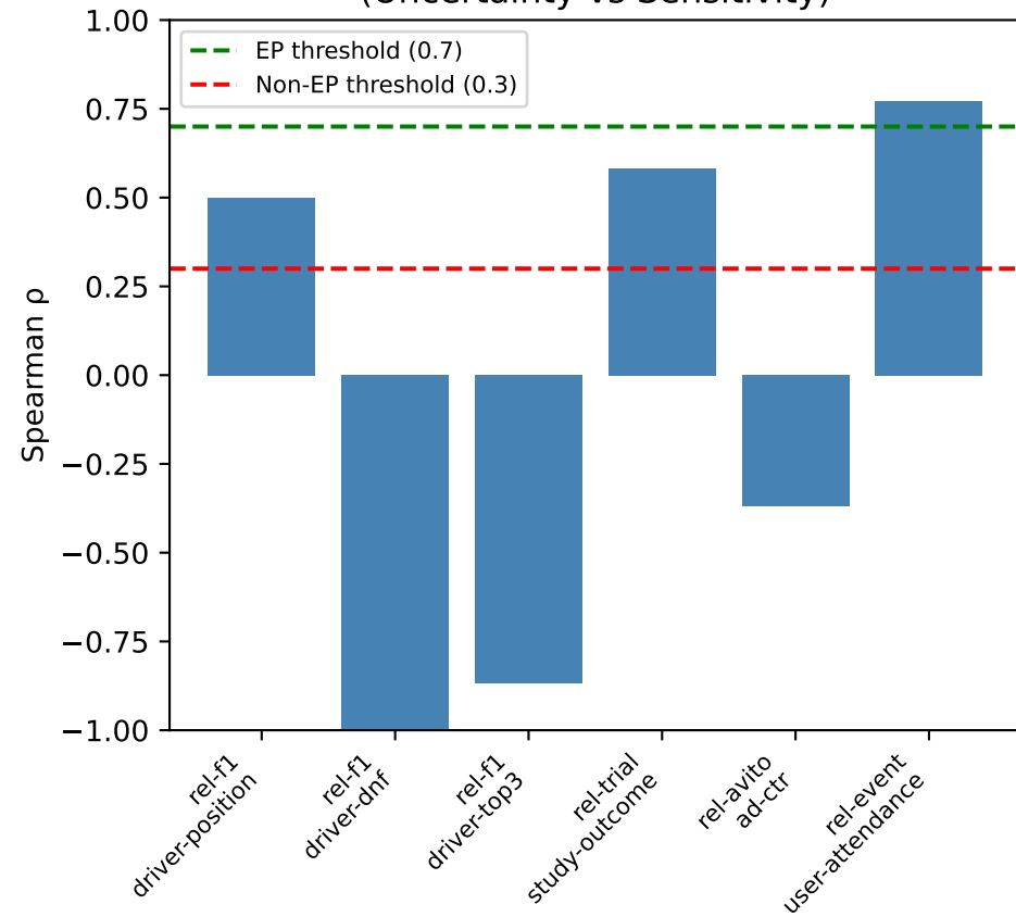
Corruption Experiment (Uncertainty vs Sensitivity)
