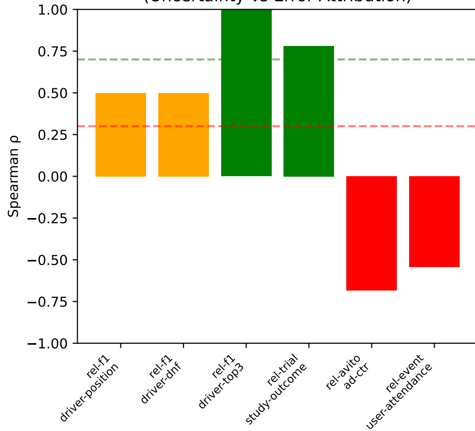
EP Detection (Uncertainty vs Error Attribution)
