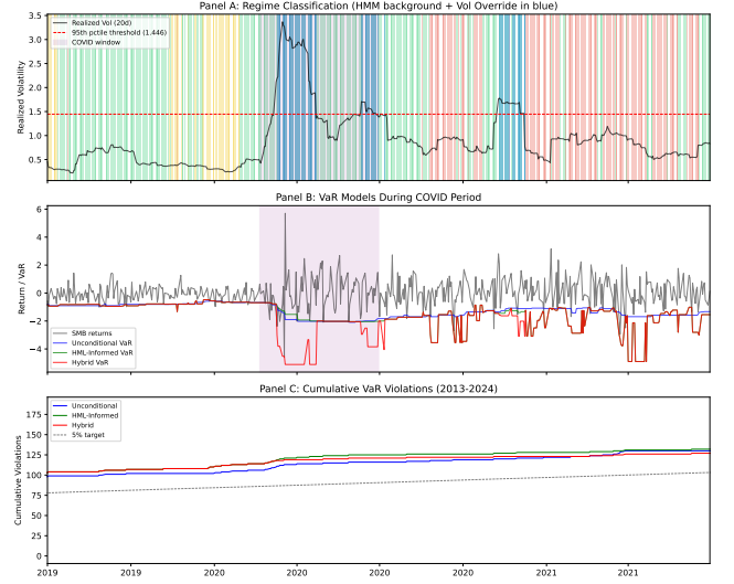
Figure 4: Hybrid detector performance. Panel A: realized volatility with 95th percentile threshold and override periods (COVID window highlighted). Panel B: SMB returns with unconditional, HML-informed, and hybrid VaR. Panel C: cumulative violations vs. 5% target.
