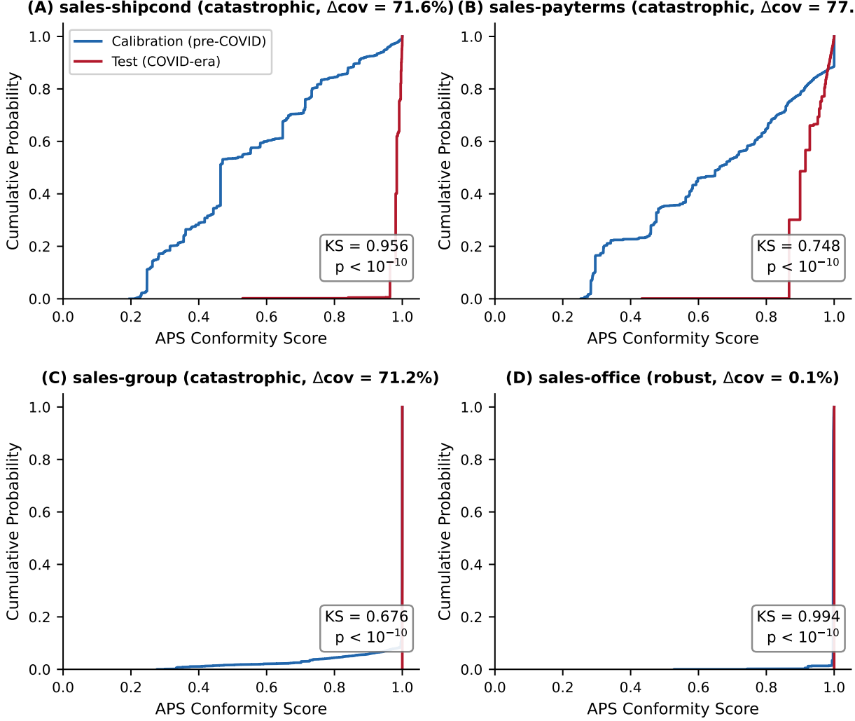
Figure 3: Conformity score CDFs (seed=42). Catastrophic tasks show rightward test-score shifts (stochastic dominance), while robust tasks can show near-degenerate or left-shift behavior.
