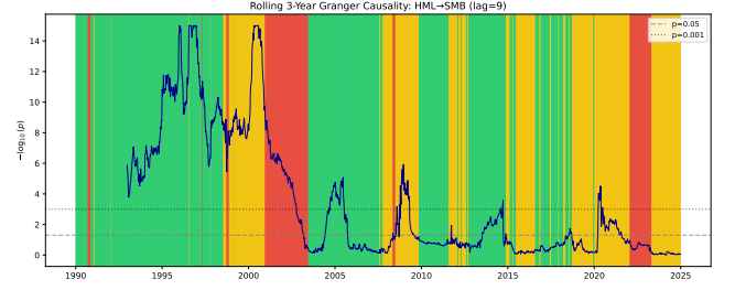
Figure 5: Rolling 3-year unconditional Granger causality ( -\log_{10}(p) , HML \rightarrow SMB, lag=9). Background shading shows HMM regime assignments for reference. Predictive strength varies episodically, with peaks during periods overlapping known market stress events. This rolling analysis does not condition on regime labels; regime-conditional results are in Table 3.
