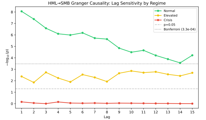
Figure 6: Granger causality p -values for HML \rightarrow SMB across lags 1–15 by regime. Normal regime (green) shows concentrated short-lag significance ( p < 10^{-8} at lag 1). Crisis regime (red) remains non-significant across the tested lag range.
