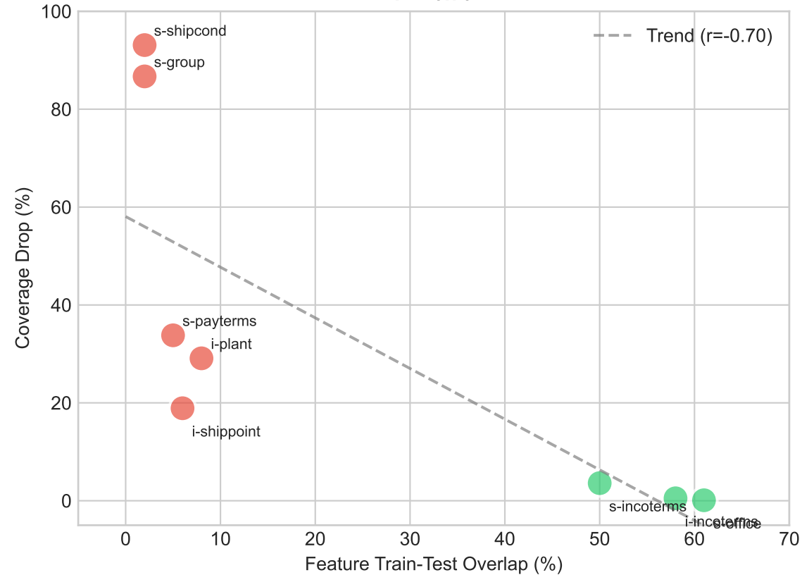
D. Feature Stability Predicts Failure r = -0.70
