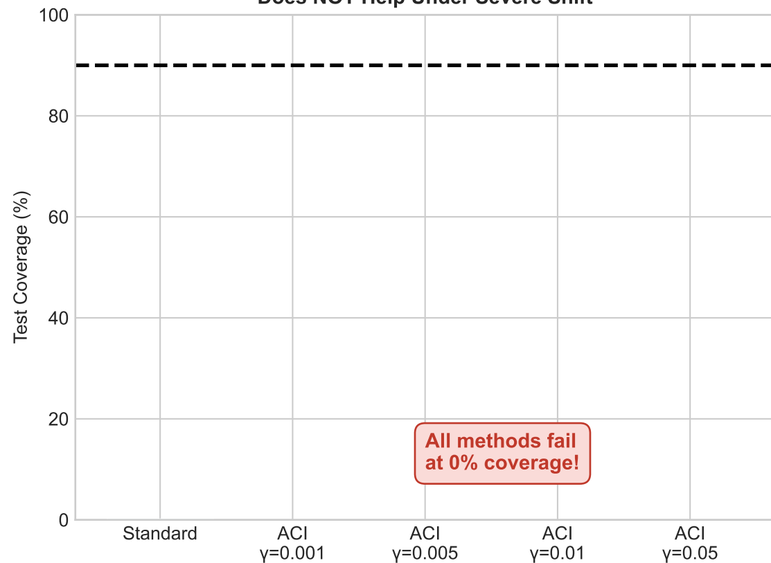
A. Adaptive Conformal Inference (ACI) Does NOT Help Under Severe Shift
