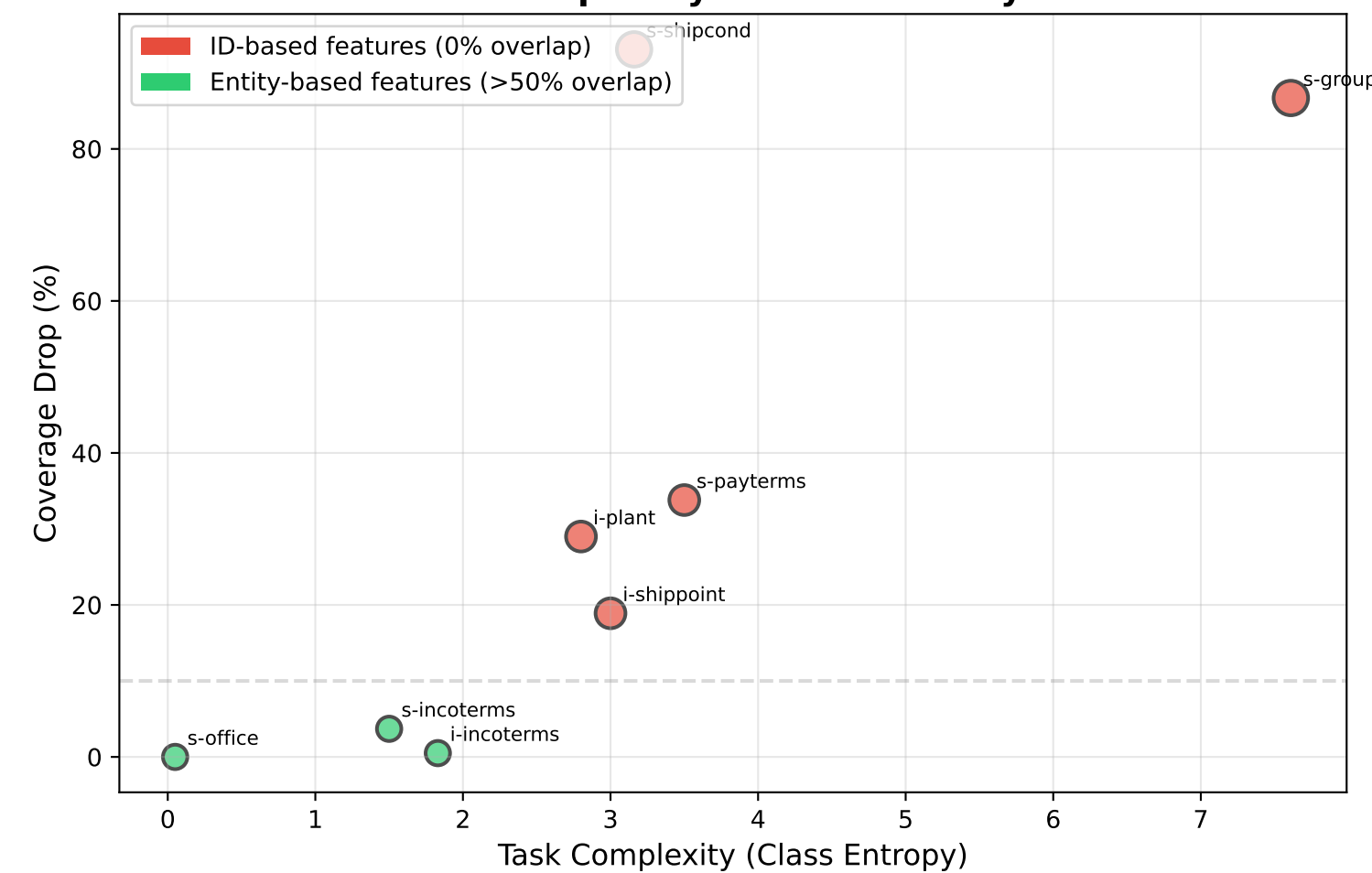
C. Complexity vs Vulnerability
