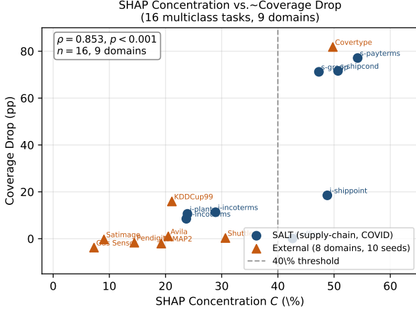
Figure 2: SHAP Concentration Correlates with Coverage Degradation (Primary Result) . Spearman \rho = 0.853 , p < 0.001 across all 16 multiclass tasks in 9 domains (dark circles: 8 SALT supply-chain tasks; orange triangles: 8 external domains, 10-seed means). The 40% threshold (dashed) is derived from validation data only. Within SALT alone: \rho = 0.833 , p = 0.010 ( n = 8 ).
