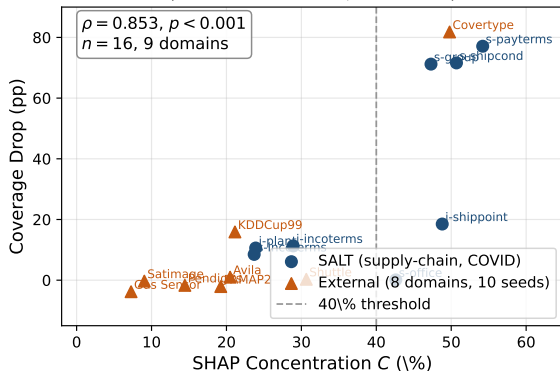
SHAP Concentration vs. ~Coverage Drop (16 multiclass tasks, 9 domains)
