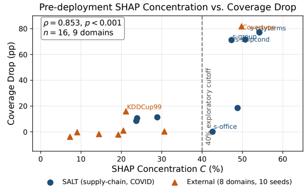
Figure 2: SHAP Concentration Correlates with Coverage Degradation (Primary Result). Spearman \rho = 0.853 , p < 0.001 across all 16 multiclass tasks in 9 domains (dark circles: 8 SALT supply-chain tasks; orange triangles: 8 external domains, 10-seed means). The 40% threshold (dashed) is an exploratory historical cutoff. Within SALT alone: \rho = 0.833 , p = 0.010 ( n = 8 ).
