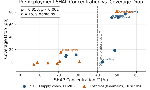
Figure 2: Historical Summary Association (Original Runs Unverified) . Spearman \rho = 0.853 , p < 0.001 across all 16 multiclass tasks in 9 domains (dark circles: 8 SALT supply-chain tasks; orange triangles: 8 external domains, 10-seed means). The plotted pre-deployment label and 40% cutoff are historical claims, not validated prospective performance; the recovered full follow-up panel does not reproduce this positive association. Within SALT alone: \rho = 0.833 , p = 0.010 ( n = 8 ).
