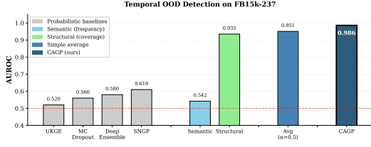
Figure 1: Temporal OOD detection (AUROC). Existing probabilistic methods achieve only 0.44–0.64; CAGP combines complementary semantic and structural signals to reach 0.94–1.00 across three benchmarks.
