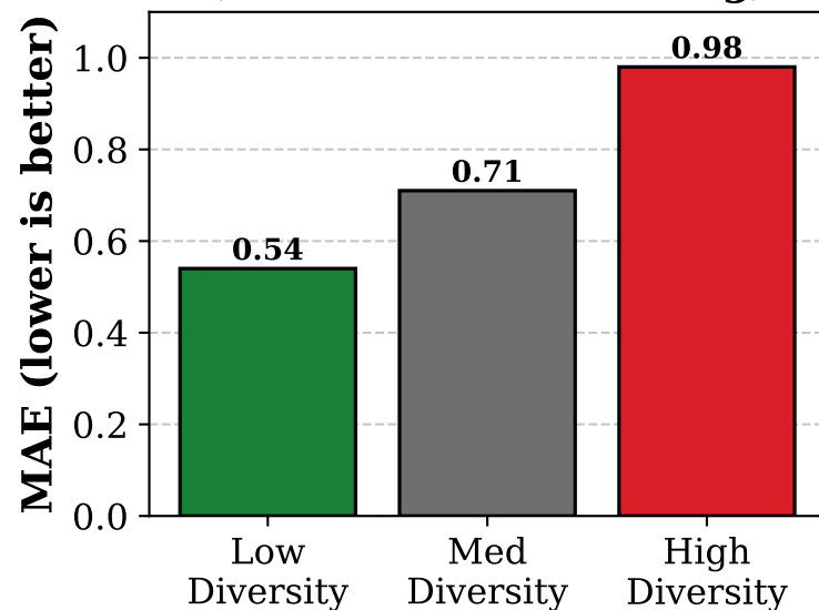
(C) MovieLens (Collaborative Filtering)
