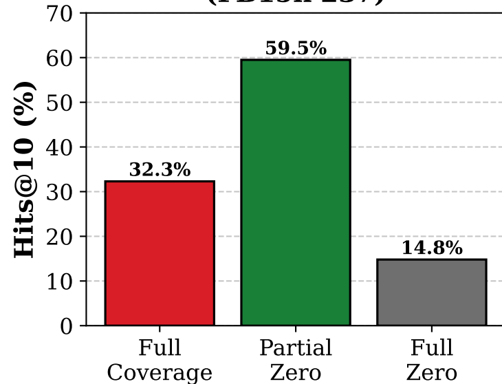
(A) Knowledge Graph (FB15k-237)
