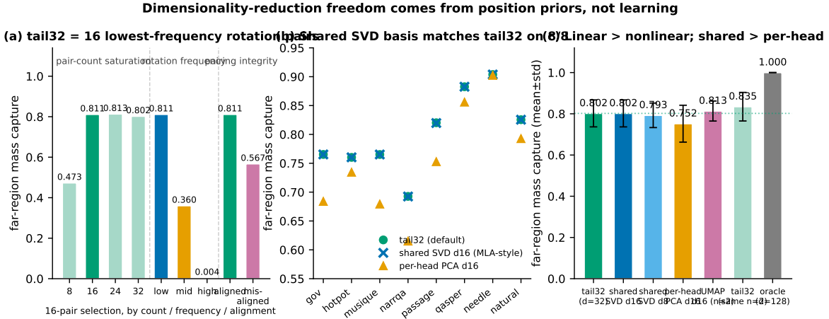
Figure 4: Dimensionality-reduction freedom comes from position priors: (a) tail32 equals the 16 complete lowest-frequency rotation pairs (frequency monotonicity, misaligned pairing collapses to 0.567, saturation at 16 pairs); (b) a shared SVD basis at d=16 matches tail32 on 8/8 samples; (c) linear beats nonlinear, shared beats per-head – UMAP was evaluated on only 2 samples (fit cost 80–167s per layer-sample), and the paired reference bar gives tail32 on the same 2 samples (0.835 versus 0.813).
