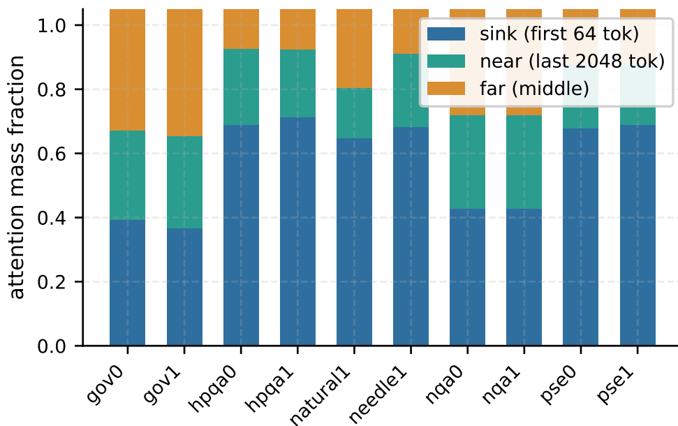
H1: position-dependent mass decomposition (Qwen3-8B, 10 traces)
