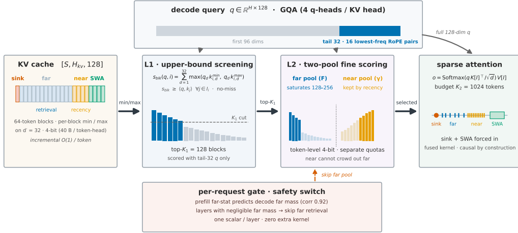
PSI: Position-Stable Indexing — training-free upper-bound block screening with far/near budget partitioning
