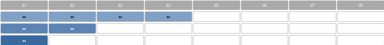
A tournament reduction over 8 segments: \log_2 n sequential rounds, every pair in a round independent. Rounds start sparse (degree-1 displacements: cheap, support-gated folds) and only the last \sim 2 \log_2 n concatenations along the critical path pay full dense-fold cost. A 1000-segment path goes from 1000 serial dense folds to 10 dense folds of dependency depth, with up to 500 independent concurrent concatenations in round 1.
