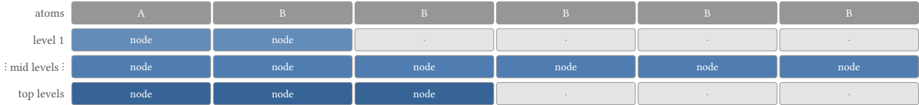
The fold DAG is a funnel : thin at the atoms and at the deepest levels, widest in the middle (2×12: 11 levels, 600 nodes, peak 150 nodes at one level). Width per level is what a parallel schedule can harvest; the barriers between levels are what it must pay.
