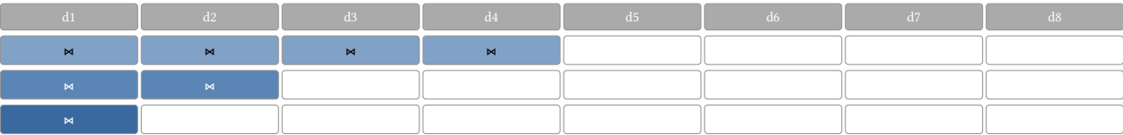
A tournament reduction over 8 segments: \log_2 n sequential rounds, every pair in a round independent. Rounds start sparse (degree-1 displacements: cheap, support-gated folds) and only the last \sim 2 \log_2 n concatenations along the critical path pay full dense-fold cost. A 1000-segment path goes from 1000 serial dense folds to 10 dense folds of dependency depth, with up to 500 independent concurrent concatenations in round 1.
