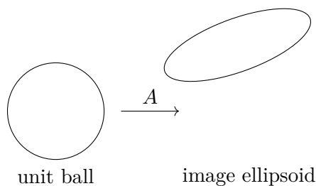
Figure 69.1: SVD describes the image of the unit ball as an ellipsoid.
