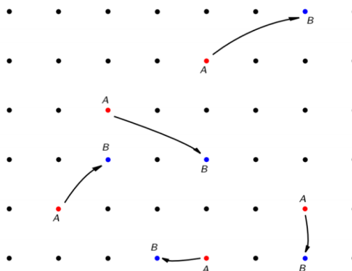
Figure 146.10: Within one orbit, equidecomposition becomes a matching problem.
