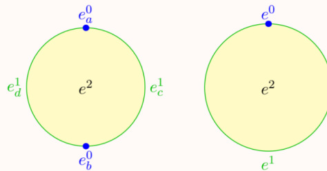
Figure 143.3: Two CW descriptions of D^2 : one more literal, one more economical.
