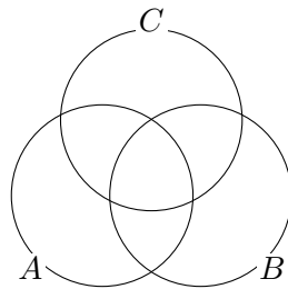
Figure 43.1: For three sets one should reason region by region, not by visual guesswork alone.
