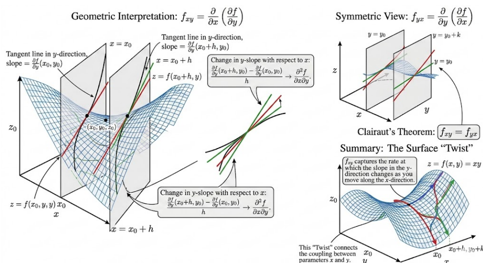
Figure 95.1: A mixed partial derivative measures how one coordinate slope changes as we move in the other coordinate direction.
