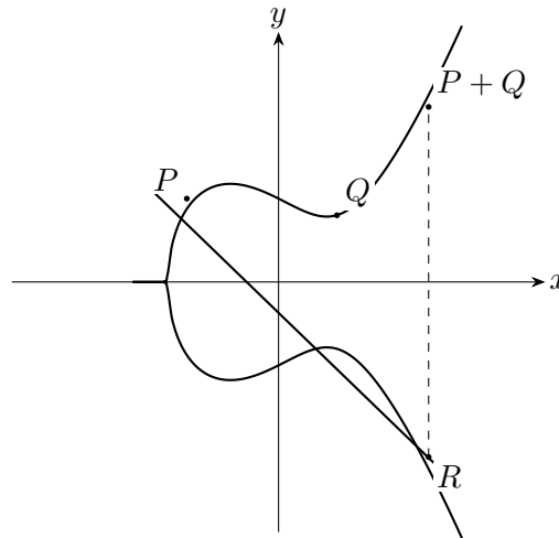
Figure 29.1: Schematic chord-and-tangent addition on an elliptic curve.
