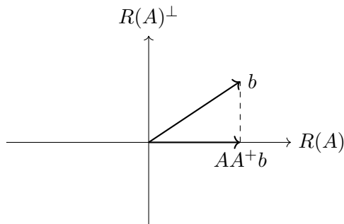
Figure 70.1: The vector AA^+b is the orthogonal projection of b onto the column space.
