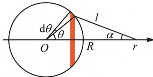
Figure 100.2: Geometry of the shell integral: the distance \ell from the field point to a surface element and the projection angle used when passing from scalar potential to radial force.
