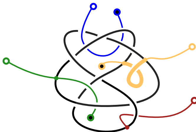
Figure 148.6: From Nikonov’s paper: probe diagrams for arc, semiarc, region, and crossing elements.
