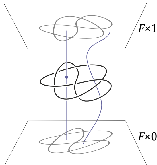
Figure 149.2: From Nikonov's paper: a region probe passes through the complement of the knot.
