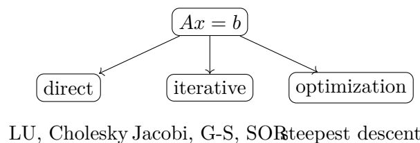
Figure 71.1: Linear systems can be solved by factorization, iteration, or minimization.
