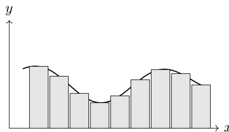
Figure 112.2: A schematic midpoint Riemann sum. The exact picture is less important than the limiting idea.
