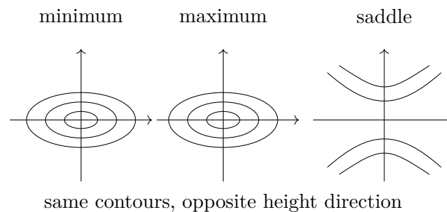
Figure 98.1: Near a nondegenerate critical point, the Hessian determines the local quadratic shape.
