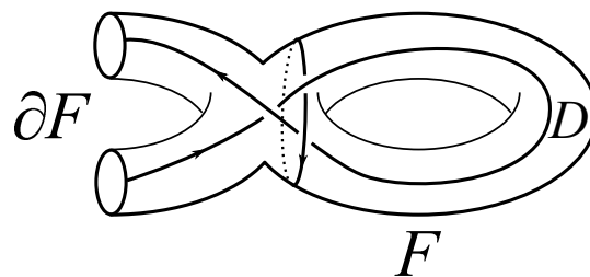
Figure 148.2: From Nikonov’s paper: a tangle diagram on a surface.
