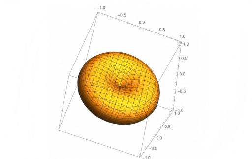
Figure 109.2: A torus as a standard example of a parametrized surface.
