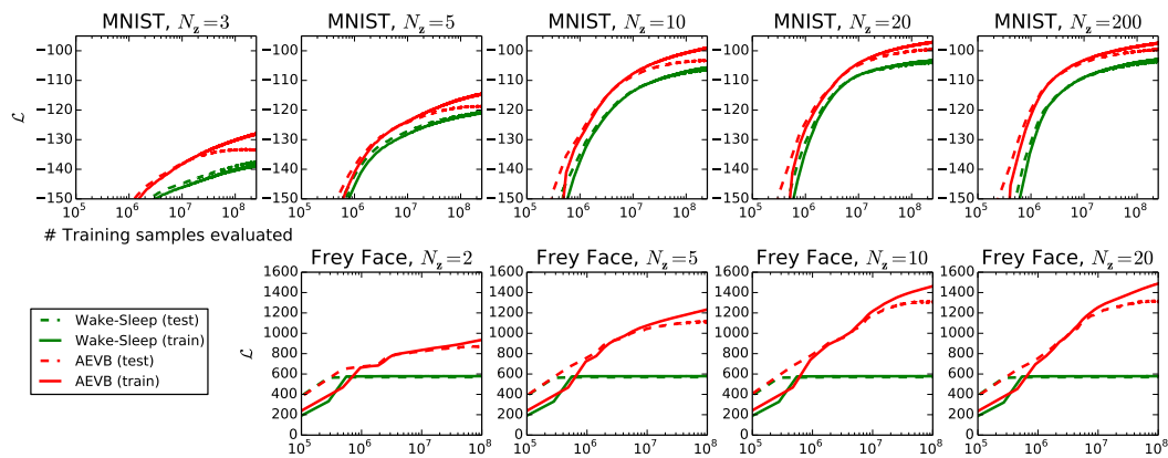
Figure 153.1: Variational lower bound curves in the AEVB experiments.
