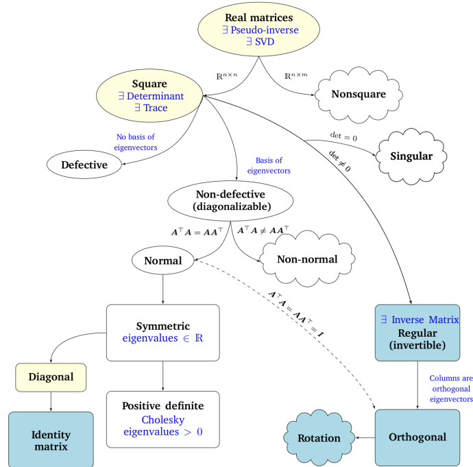
Figure 64.8: A functional phylogeny of real matrices encountered in machine learning, indicating which tools apply to which matrix classes.
