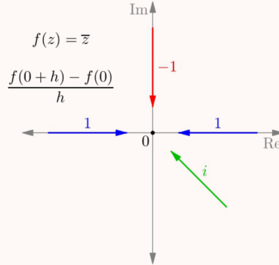
Figure 111.1: In complex differentiability, the increment approaches from all directions in the plane.
