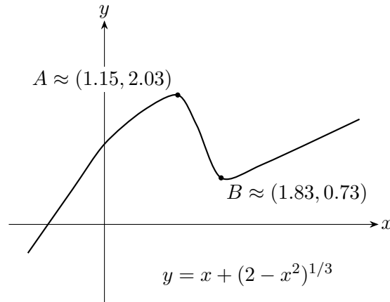
Figure 72.1: Reconstruction of the graph used for the constrained extremum problem.
