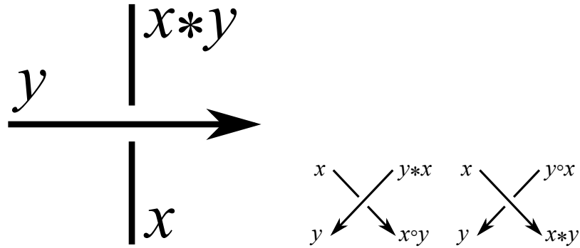
Figure 149.1: From Nikonov's paper: arc and semiarc colorings are the neighbouring examples around the region story.
