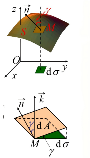
Figure 109.1: A surface area element and its projection. The factor between dS and the projected area element is determined by the angle between the surface normal and the projection direction.
