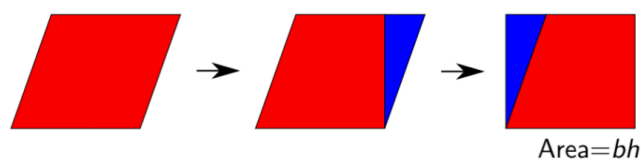
Figure 146.1: A parallelogram dissected and rearranged into a rectangle.
