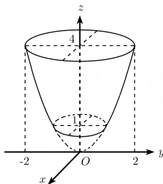
Figure 106.2: A rotational solid with circular cross-sections at different heights. Such diagrams are read by projecting to the base plane and then recovering the vertical bounds.
