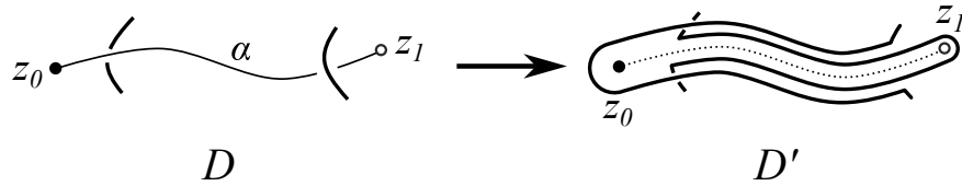
Figure 149.6: From Nikonov’s paper: clearing a region probe in the construction of the partial tribracket.
