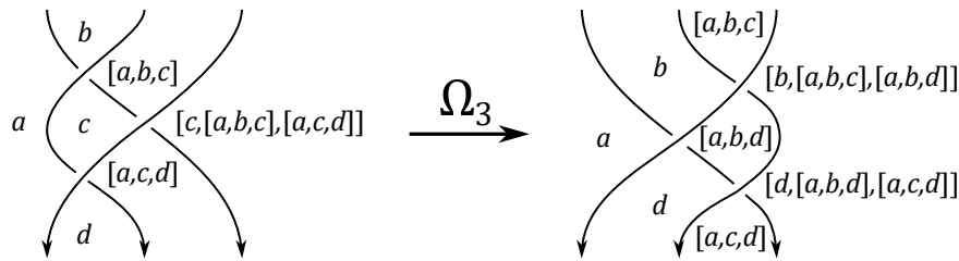
Figure 149.4: From Nikonov's paper: the third Reidemeister move is the source of the tribracket identity.
