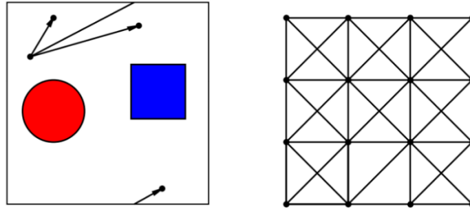
Figure 146.9: The generator graph: locally it looks like a lattice with bounded moves.
