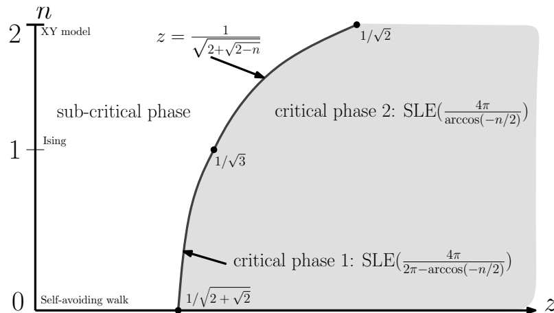
Figure 50.4: phase diagram for O(n) loop models.
