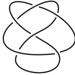
Figure 148.1: From Nikonov’s paper: a knot diagram. It is a planar record of a three-dimensional object.
