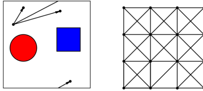
Figure 125.9: The generator graph: locally it looks like a lattice with bounded moves.
