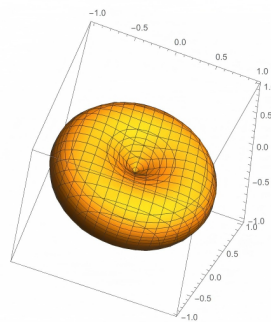
Figure 98.2: A torus as a standard example of a parametrized surface.
