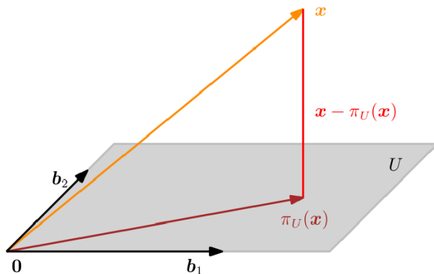
Figure 56.1: Projection onto a two-dimensional subspace: the residual x - \pi_U(x) is orthogonal to the basis directions of U .
