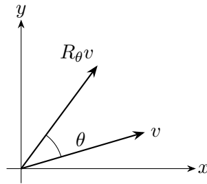
Figure 43.1: A planar rotation acts linearly on vectors and is represented by R_\theta .
