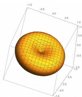
Figure 105.2: A torus as a standard example of a parametrized surface.
