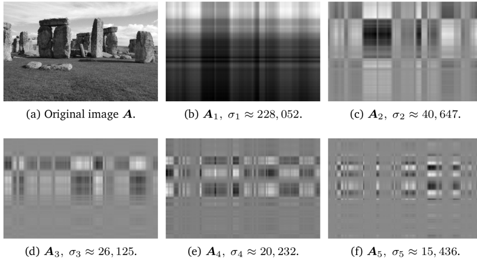
Figure 58.6: The first rank-one SVD components of an image. Each component captures one weighted visual pattern rather than a recognizable full image.
