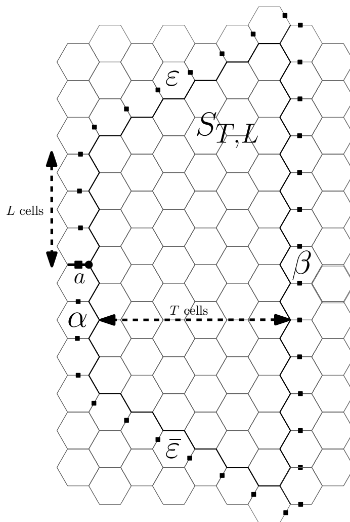
Figure 46.3: the trapezoidal domain S_{T,L} and its boundary pieces.
