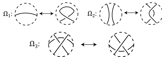
Figure 140.3: From Nikonov's paper: Reidemeister moves. These are the local equivalences that make diagrams represent knots.
