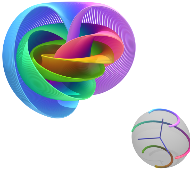
Figure 142.1: the Hopf fibration visualized by linked fibres.
