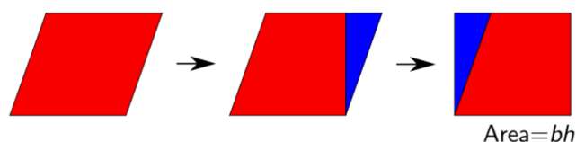
Figure 145.1: A parallelogram dissected and rearranged into a rectangle.
