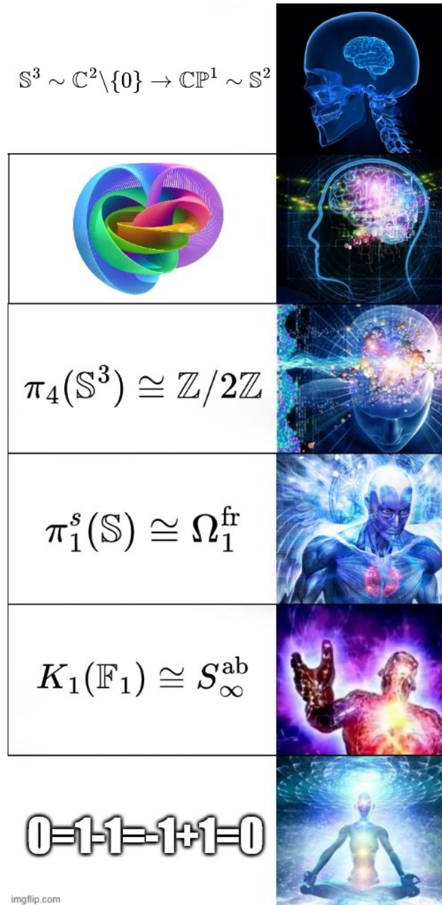
Figure 139.2: the meme that compresses Hopf fibration, stable homotopy, K -theory, and the equation 0 = 1 - 1 = -1 + 1 = 0 into one ladder.
