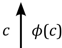
Figure 141.7: From Nikonov’s paper: a local propagation rule for neighbouring regions.
