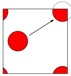
Figure 145.7: Working on the torus: translations wrap around the fundamental cube.
