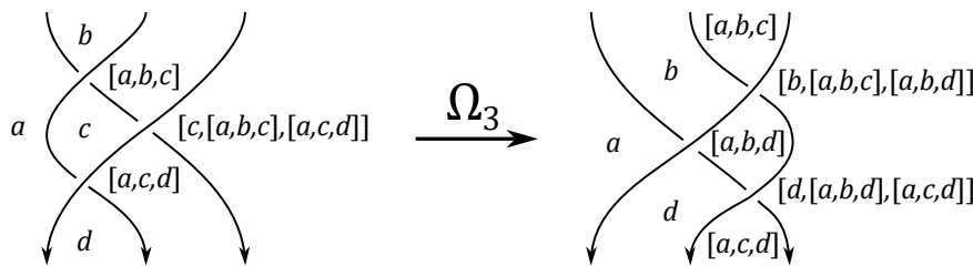
Figure 141.4: From Nikonov's paper: the third Reidemeister move is the source of the tribracket identity.
