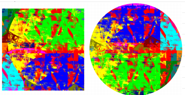
Figure 145.12: A visual impression of the Borel circle-squaring pieces.
