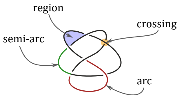
Figure 140.4: From Nikonov’s paper: the elementary pieces of a knot diagram.
