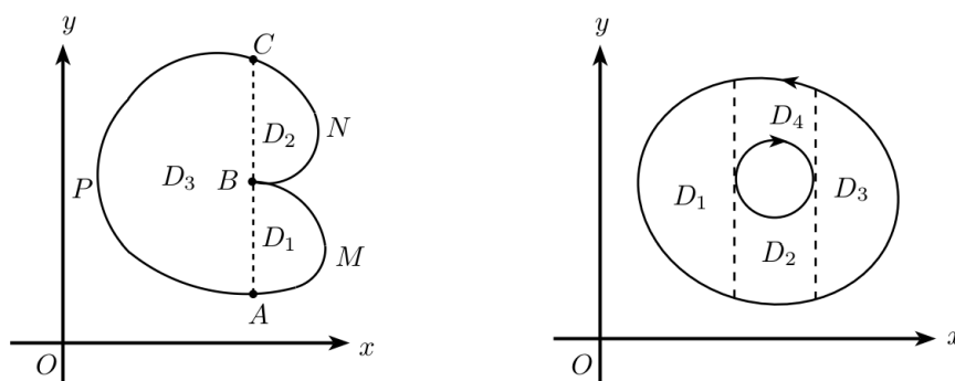
Figure 99.3: Subdivision by auxiliary arcs: internal boundary contributions cancel, leaving only the outer boundary.
