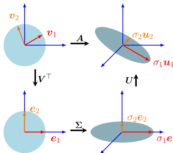
Figure 58.4: Geometric interpretation of SVD: the unit disk is first expressed in the right-singular-vector coordinates, then stretched by the singular values, and finally rotated into the output coordinates.
