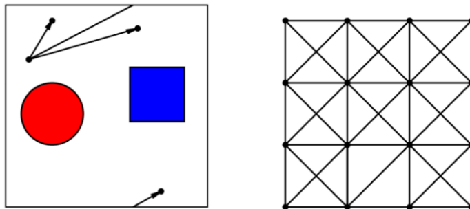
Figure 145.9: The generator graph: locally it looks like a lattice with bounded moves.
