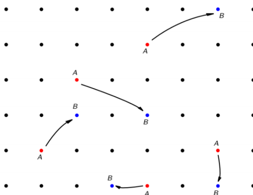
Figure 145.10: Within one orbit, equidecomposition becomes a matching problem.
