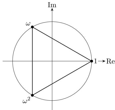
Figure 100.2: Primitive third roots of unity on the unit circle. Divisibility by x^2 + x + 1 is checked by evaluating at \omega and \omega^2 .
