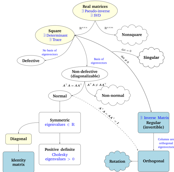
Figure 58.8: A functional phylogeny of real matrices encountered in machine learning, indicating which tools apply to which matrix classes.
