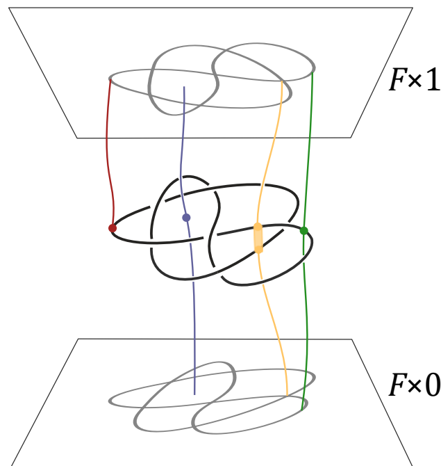
Figure 140.5: From Nikonov's paper: topological interpretation of diagram elements by probes in F \times I .
