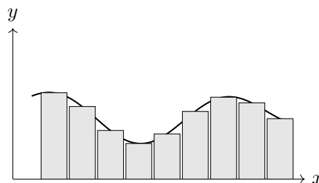
Figure 102.2: A schematic midpoint Riemann sum. The exact picture is less important than the limiting idea.
