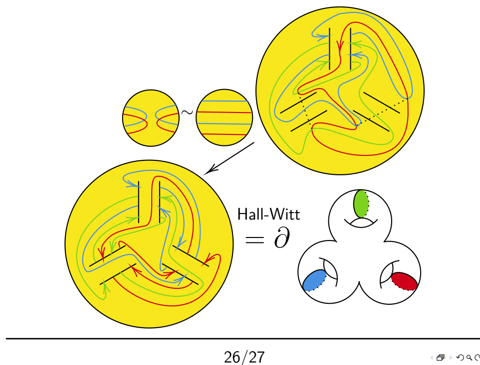
Figure 142.8: From the lecture slides: the boundary relation for the three-lasagna construction.
