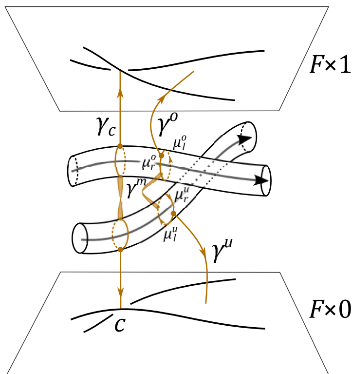
Figure 141.8: From Nikonov's paper: a crossing probe. Crossings are treated as probe classes rather than merely as vertices of a drawing.
