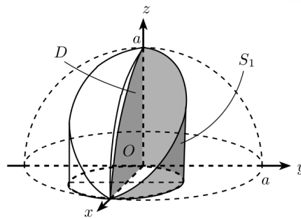
Figure 105.4: A related spherical surface cut out by a vertical boundary. The dashed curves indicate the hidden projection and bounding geometry.
