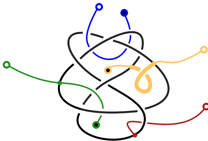
Figure 140.6: From Nikonov’s paper: probe diagrams for arc, semiarc, region, and crossing elements.
