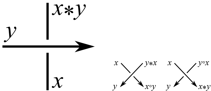
Figure 141.1: From Nikonov's paper: arc and semiarc colorings are the neighbouring examples around the region story.
