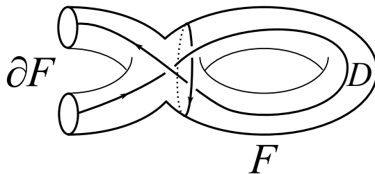
Figure 140.2: From Nikonov’s paper: a tangle diagram on a surface.
