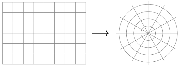
Figure 81.1: Schematic reconstruction: a rectangular grid is deformed into orthogonal curve families by a holomorphic map.
