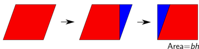
Figure 139.1: A parallelogram dissected and rearranged into a rectangle.
