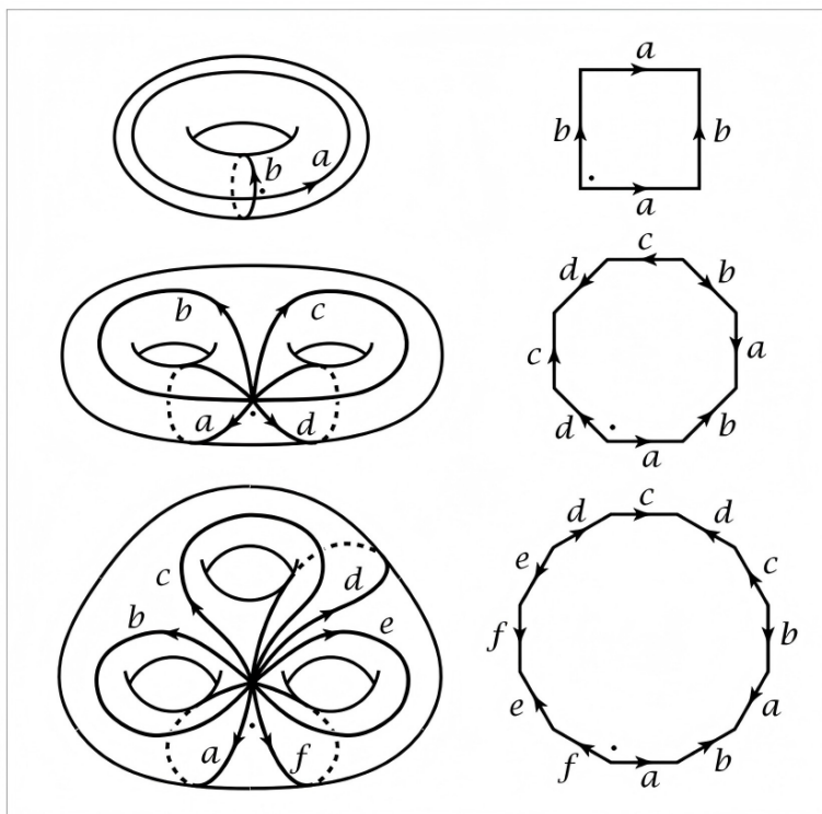
Figure 134.6: Polygon schemata and surface gluings: topology encoded by labelled boundary words.
