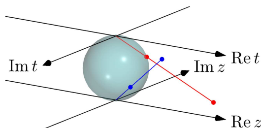
Figure 121.1: The Riemann sphere is the complex plane plus one point at infinity.
