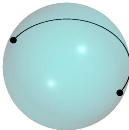
Figure 122.1: A curve carries both topology and analytic data. Divisors are one way to connect them.
