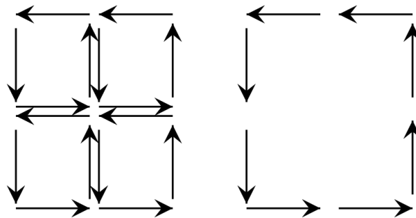
Figure 118.1: A small oriented patch: the boundary orientation is part of the theorem.
