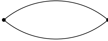
Figure 151.2: the bubble diagram.
