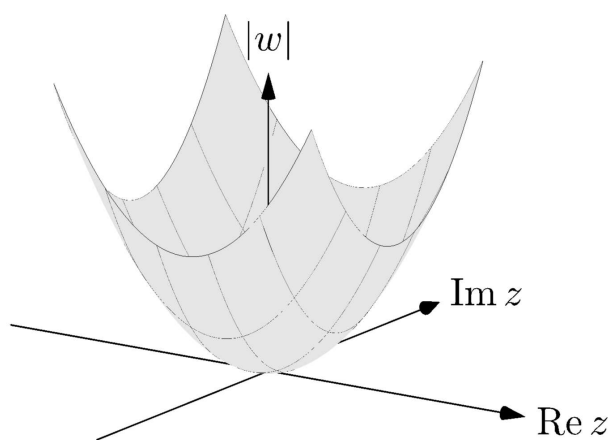
Figure 120.1: A familiar curve can be treated as an equation, not only as a picture.
