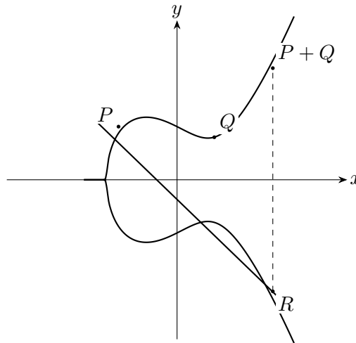
Figure 26.1: Schematic chord-and-tangent addition on an elliptic curve.
