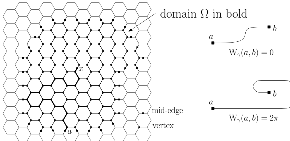
Figure 135.1: a hexagonal-lattice domain and the winding of a self-avoiding walk.
