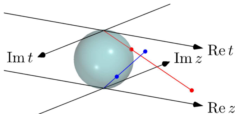
Figure 118.3: The second stereographic chart and the transition coordinate near infinity.
