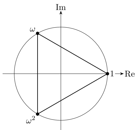
Figure 63.2: Primitive third roots of unity on the unit circle. Divisibility by x^2 + x + 1 is checked by evaluating at \omega and \omega^2 .
