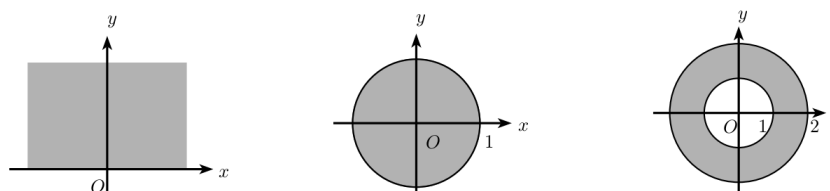
Figure 98.2: Simply connected and multiply connected plane regions. The distinction matters for path independence and conservative fields.
