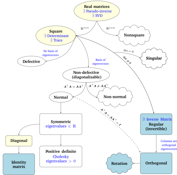
Figure 56.8: A functional phylogeny of real matrices encountered in machine learning, indicating which tools apply to which matrix classes.
