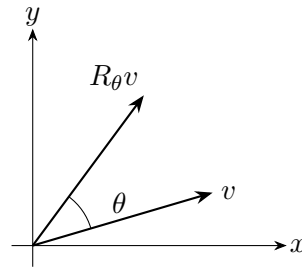
Figure 44.1: A planar rotation acts linearly on vectors and is represented by R_\theta .
