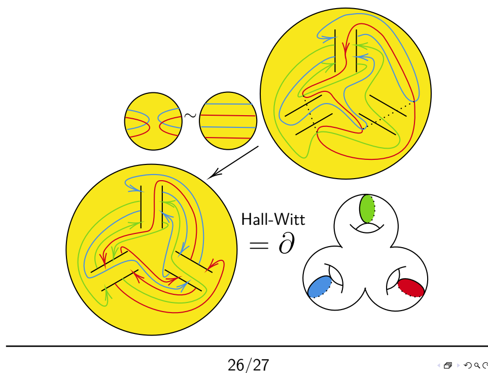
Figure 127.8: From the lecture slides: the boundary relation for the three-lasagna construction.
