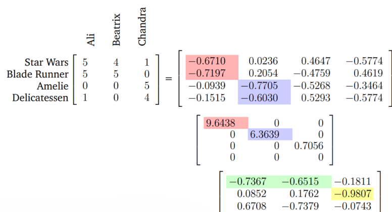
Figure 56.5: A movie-rating matrix and its SVD decomposition. Dominant singular directions highlight latent structure in user and movie preferences.
