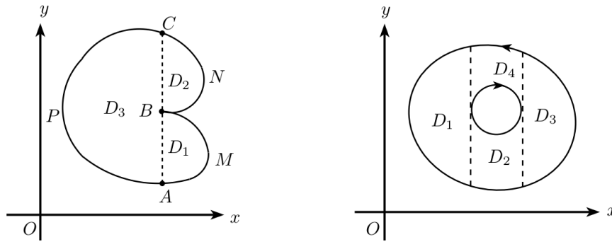
Figure 98.3: Subdivision by auxiliary arcs: internal boundary contributions cancel, leaving only the outer boundary.
