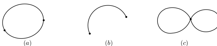
Figure 98.1: Simple closed curves and non-simple closed curves in the statement of Green's theorem.
