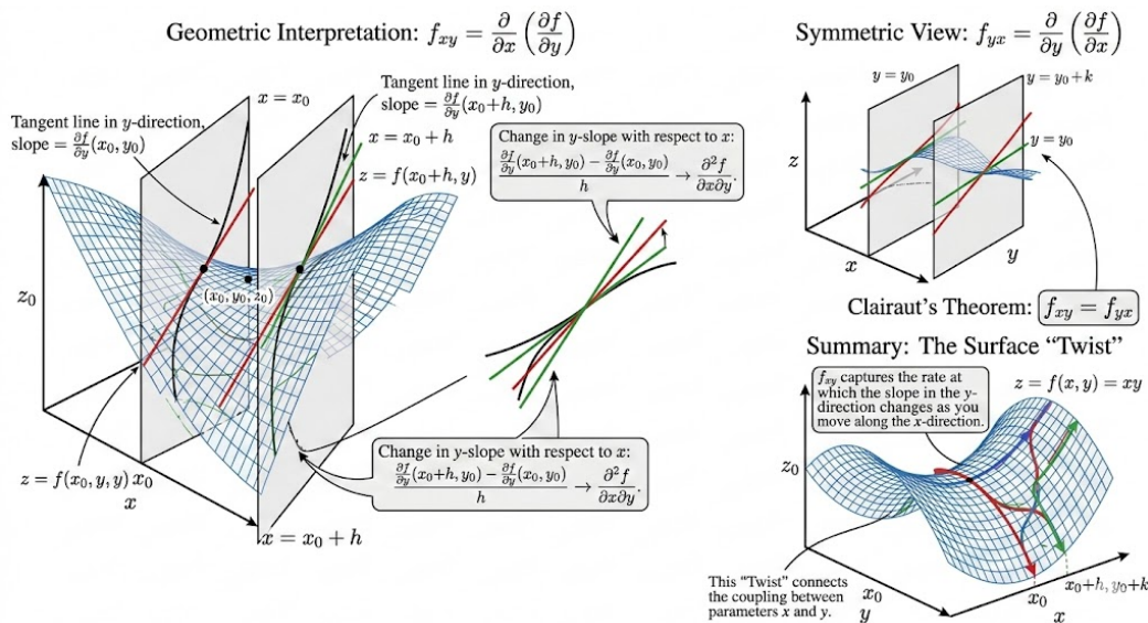
Figure 89.1: Geometric interpretation of the mixed partial derivative: it measures how the y -direction slope changes as one moves in the x -direction, and symmetrically for f_{yx} .
