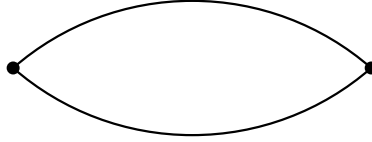
Figure 136.2: the bubble diagram.
