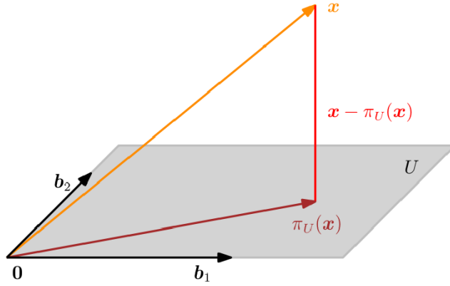
Figure 57.1: Projection onto a two-dimensional subspace: the residual x - \pi_U(x) is orthogonal to the basis directions of U .
