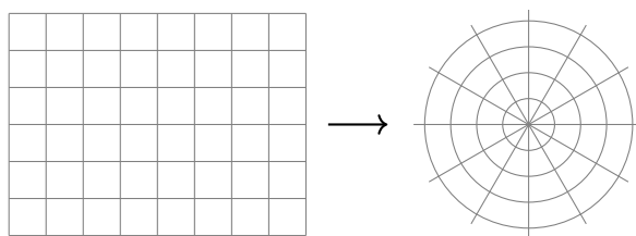
Figure 1.1: Schematic reconstruction: a rectangular grid is deformed into orthogonal curve families by a holomorphic map.
