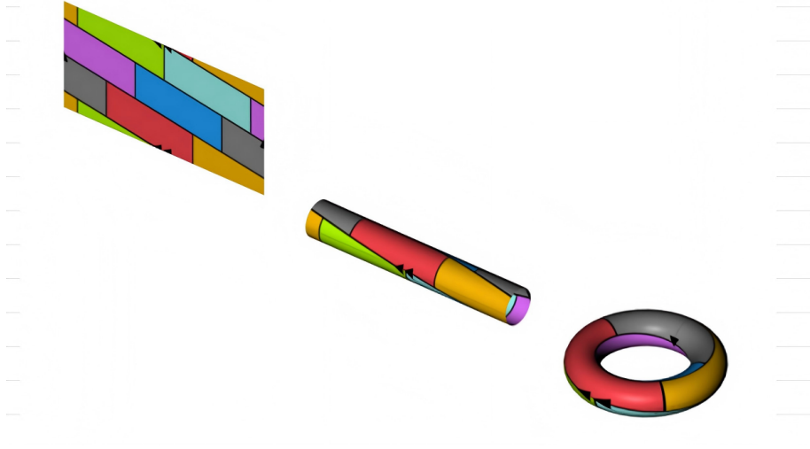
Figure 1.4: The quotient square/cylinder/torus picture: (\mathbb{R}/\mathbb{Z})^2 as a glued square.
