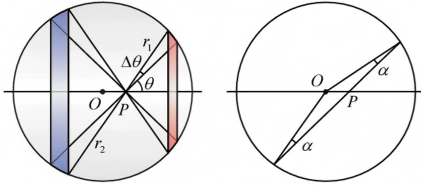
Figure 1.1: The geometric cancellation proof: the same narrow cone from an interior point cuts two opposite shell patches, and the equal angle geometry supplies the common obliquity factor.
