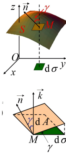
Figure 112.1: A surface area element and its projection. The factor between dS and the projected area element is determined by the angle between the surface normal and the projection direction.
