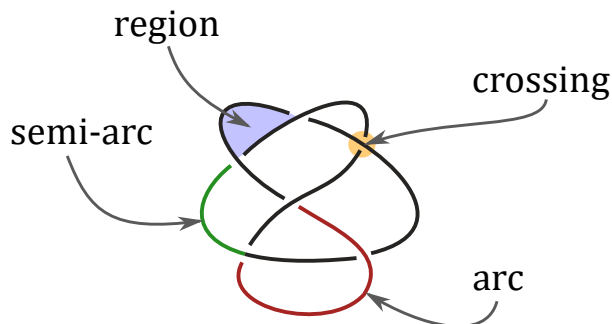
Figure 142.4: From Nikonov's paper: the elementary pieces of a knot diagram.
