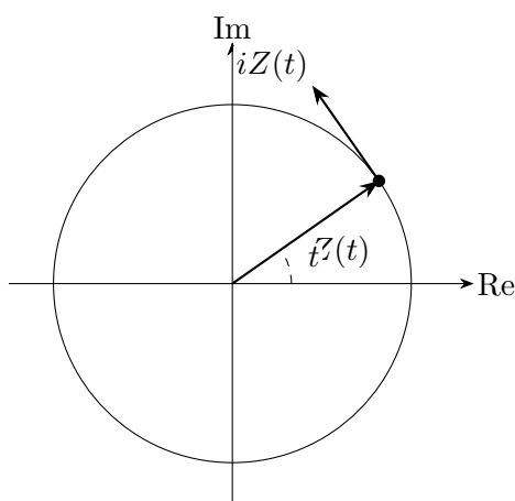
Figure 1.1: The equation Z' = iZ rotates the radius vector by 90^\circ , producing tangent velocity of constant length.
