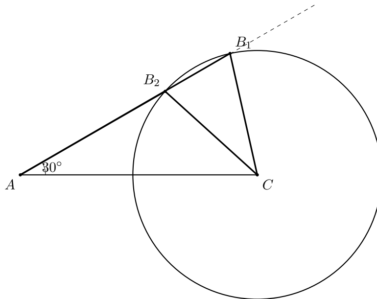
Figure 1.2: A ray from A can meet the circle centered at C twice. The two intersections are the two SSA triangles.
