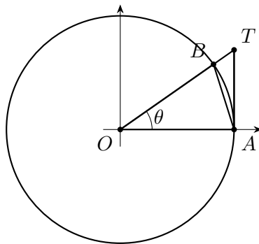
Figure 1.1: The areas of \triangle OAB , sector OAB , and \triangle OAT give \sin \theta < \theta < \tan \theta .
