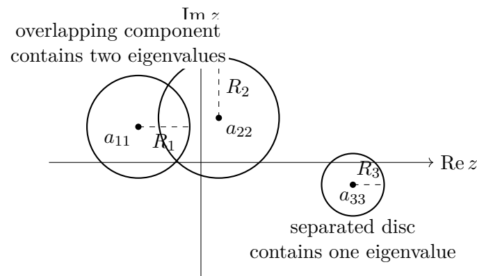
Figure 1.1: A separated component containing exactly m Gershgorin discs contains exactly m eigenvalues, counted with algebraic multiplicity.
