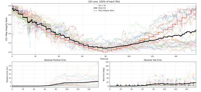
Fig. 3. Top: ESI vs map integrity ratio for default AMCL. Red = Ground truth (MIRA). Bottom left: Position error. Bottom right: Yaw error. Black = interpolated mean of the ESI, position error and yaw error, respectively.
