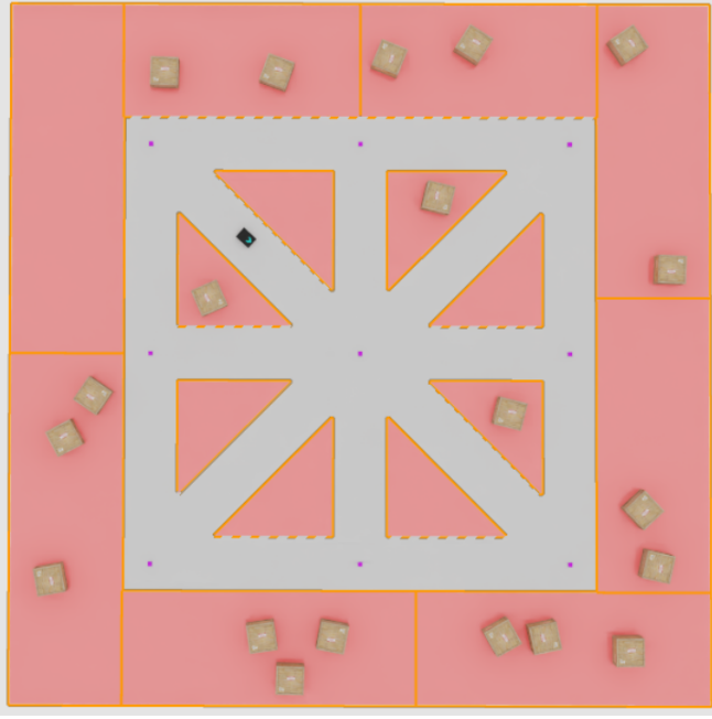
Fig. 2. Scene from Isaac Sim. Red polygons represent the obstacle space. Waypoints are marked with purple squares. The robot is seen moving from top left to center.
