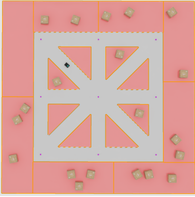
Fig. 4. Scene from Isaac Sim. Red polygons represent the obstacle space. Waypoints are marked with purple squares. The robot is seen moving from top left to center.
