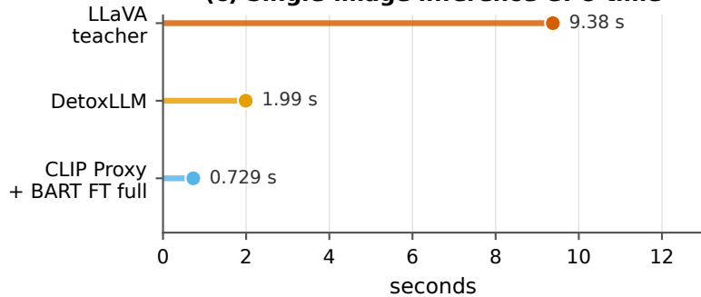
(c) Single-image inference GPU time
