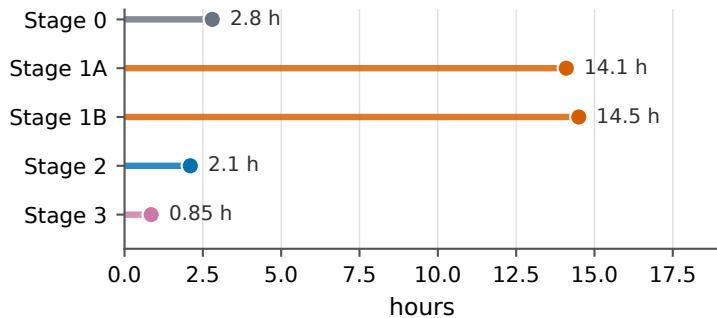
(a) Training pipeline GPU time
