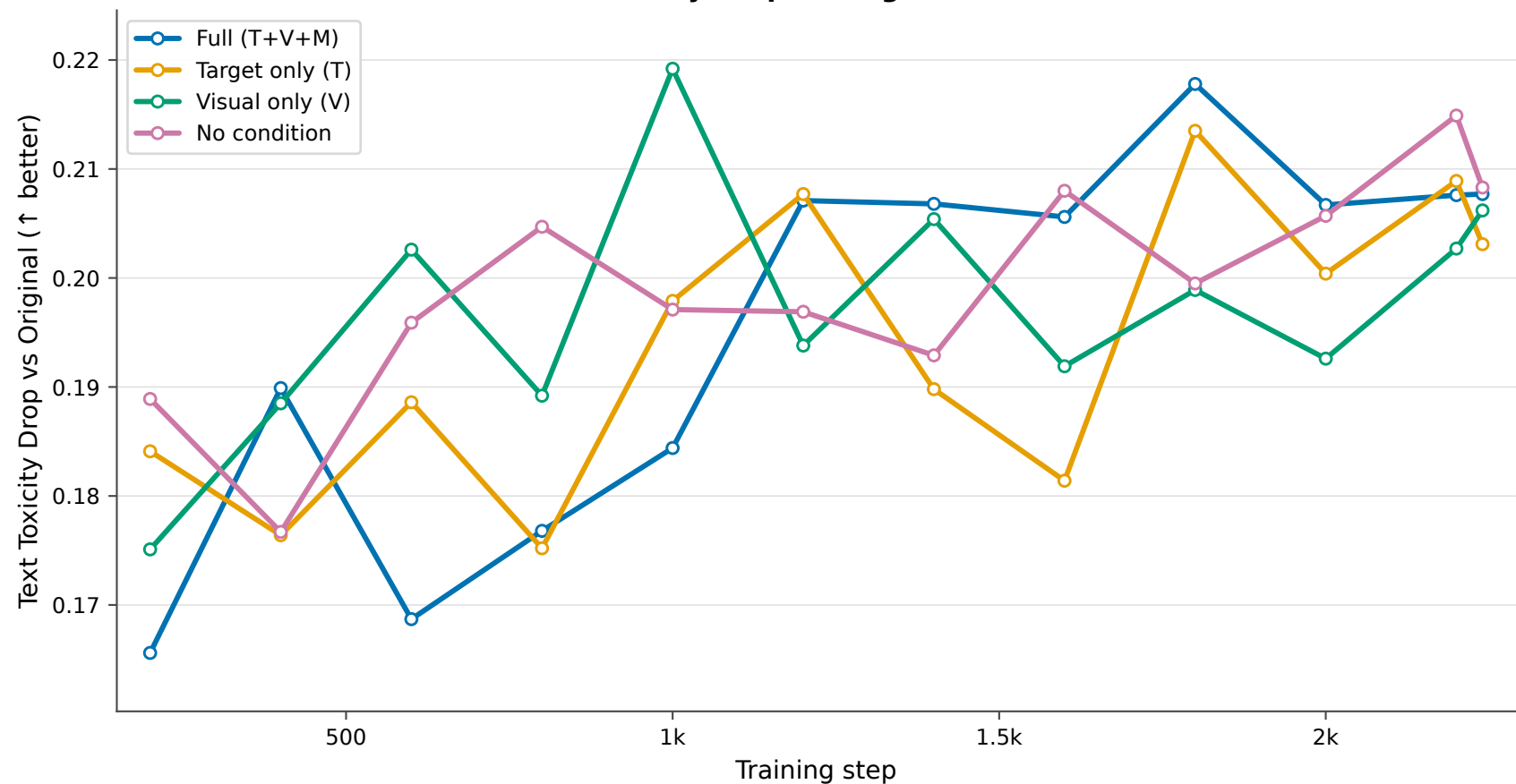
Text Toxicity Drop vs Original ( \uparrow better)
