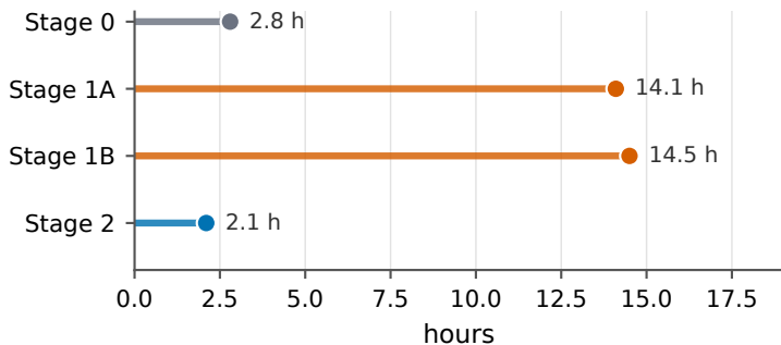
(a) Pipeline GPU time
