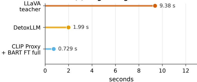
(c) Single-image GPU time
