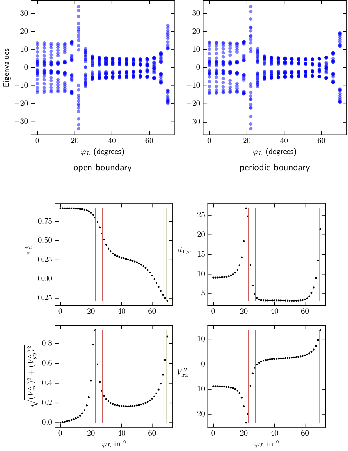
Figure 1: The occurrence of topological states is signaled by the vertical lines. Between the two red as well as between the two green lines topological states can be found.
