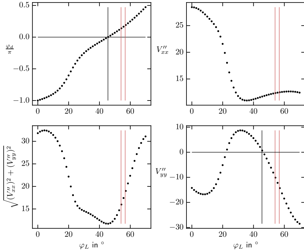
Figure 2: Topological states can again be found in the angle range between the two red vertical lines.
