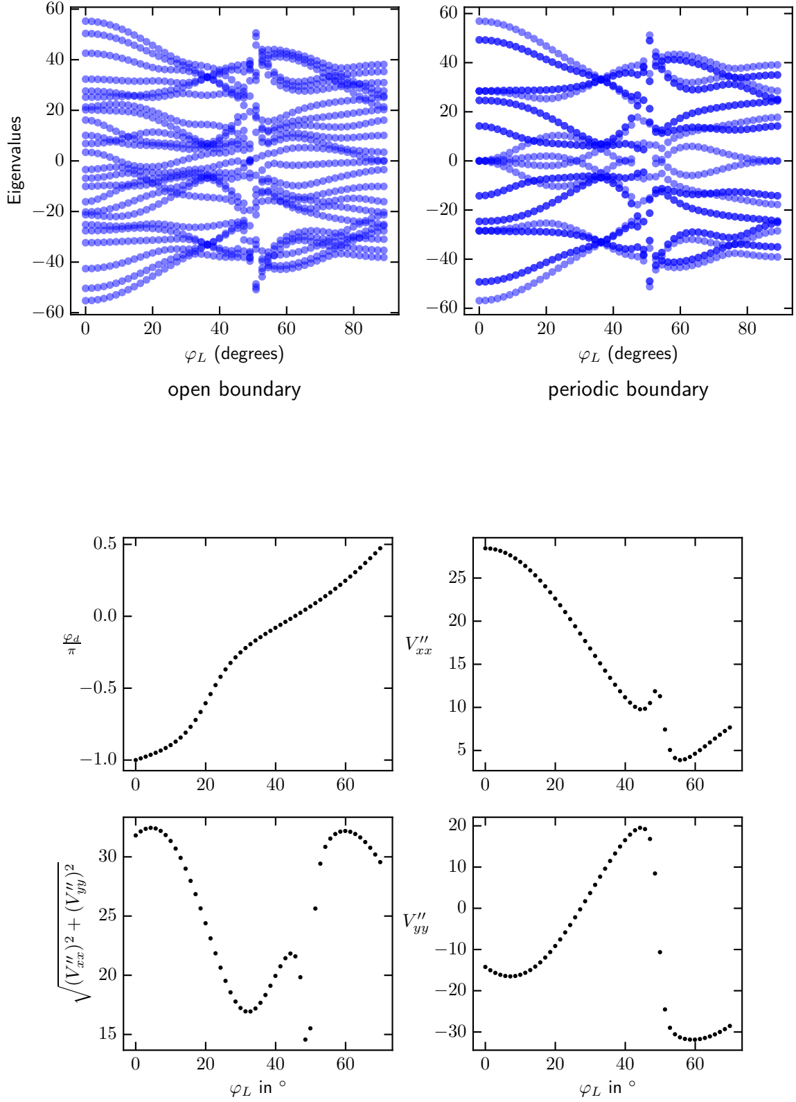
Figure 3: In this configuration with equal spacing between the atoms no topological states occur.
