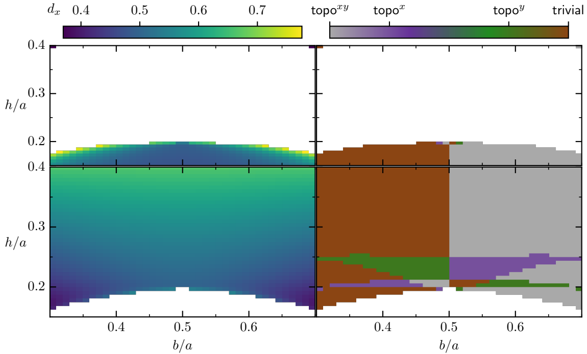
Figure 2.6: Topological phase diagram. There are up to four possible dipole orientations that decouple x and y -directions. Two of them are shown on the left panels by depicting the x -component of the dipole. White space indicates here that there were no appropriate dipoles found. On the right side of the panel the topological phases are depicted. It is shown, whether a topological phase arises for the x , y or both directions, or if the system exhibits a topologically trivial phase.
