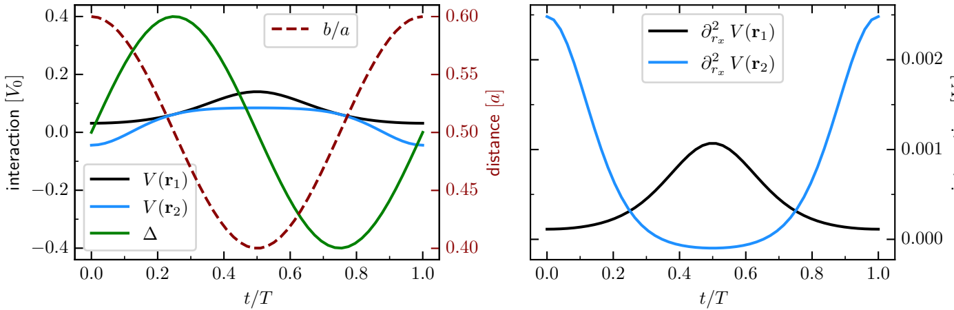
Figure 15: Rice-Mele scheme. Depicted is the course of the the decisive parameters during the Rice-Mele cycle, i.e. the axial distance between atoms in the unit cell b = 1.8\text{--}1.2\text{--}1.8r_0 (the distance orthogonal to the chain axis is kept constant h = 0.4r_0 as well as the distance inside a sublattice a = 3r_0 ). The detuning takes it's maximal value at \Delta_{\max} = 0.4V_0 .
