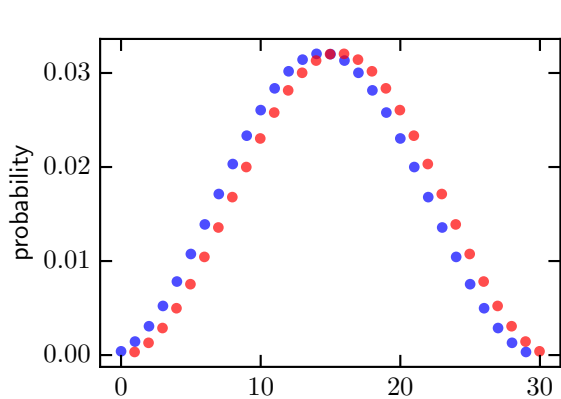
phonon direction x
