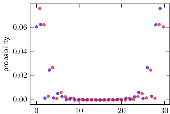
phonon direction x
