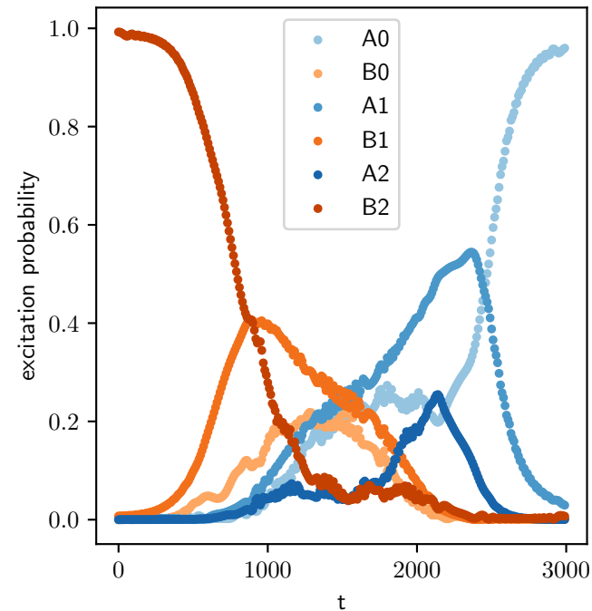
spin transport
