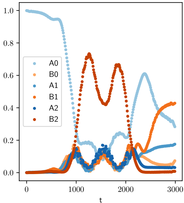
phonon transport
