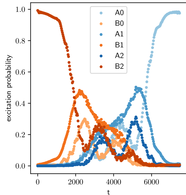
spin transport
