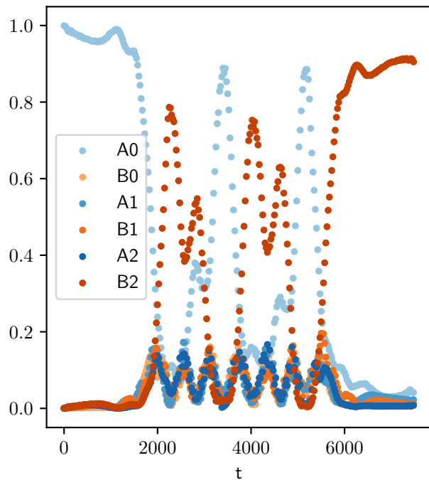
phonon transport
