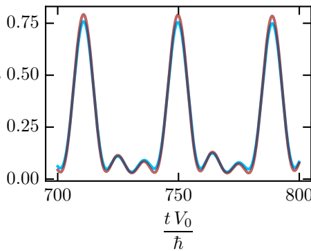
\langle a_3^\dagger a_3 \rangle
