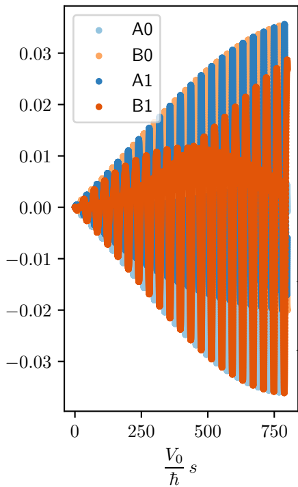
excited phonons: 3
