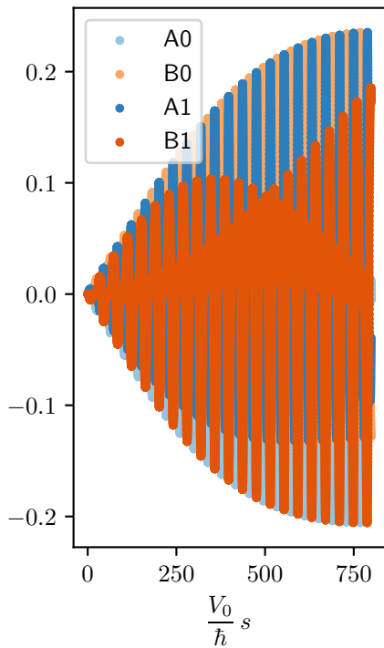
excited phonons: 12
