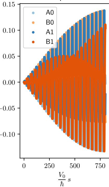
excited phonons: 7
