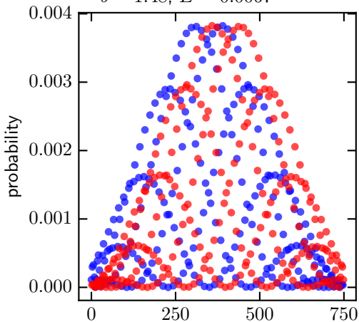
phonon direction x
