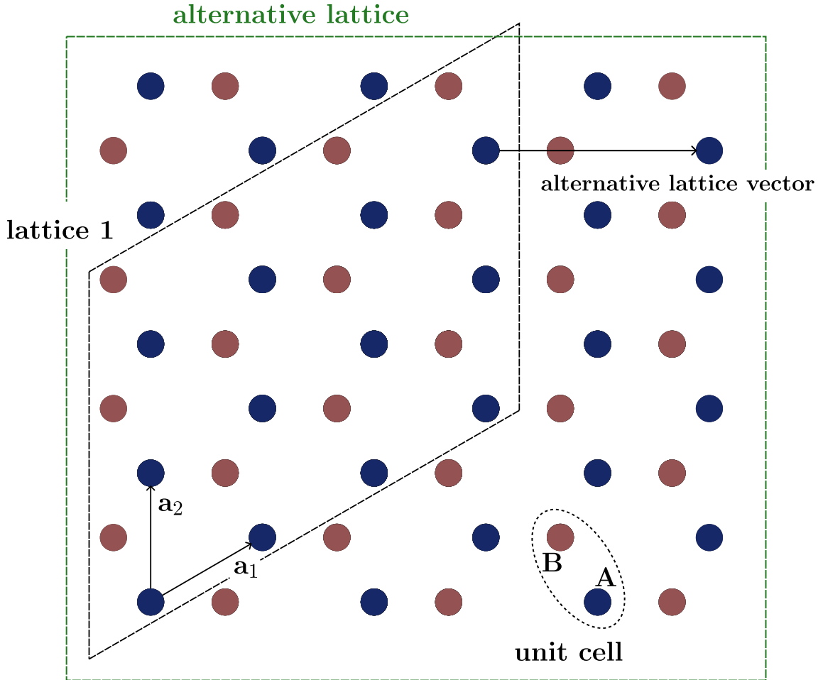
Figure 6: Lattice definition The main configuration of the grid, lattice 1, is the parallelogram spanned by the lattice vectors \mathbf{a}_1 and \mathbf{a}_2 . This is visualized by the black dashed frame. There is also the possibility of defining a square lattice which is highlighted by the green dashed frame.
