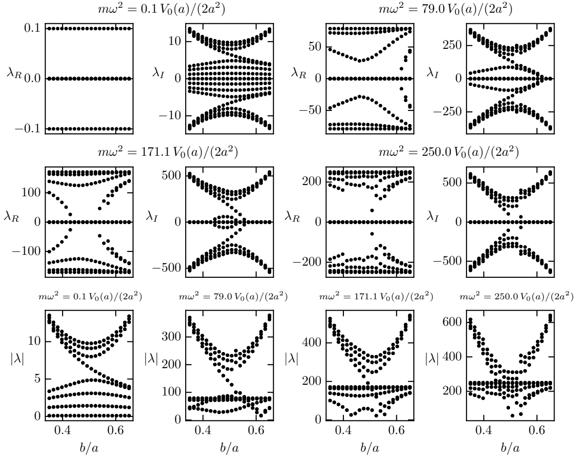
Figure 4: Spectrum of BdG Hamiltonian for different trap frequencies.
