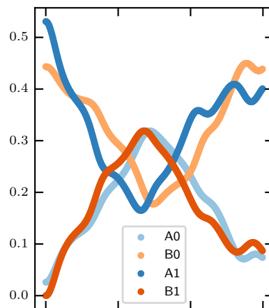
excited phonons: 10
