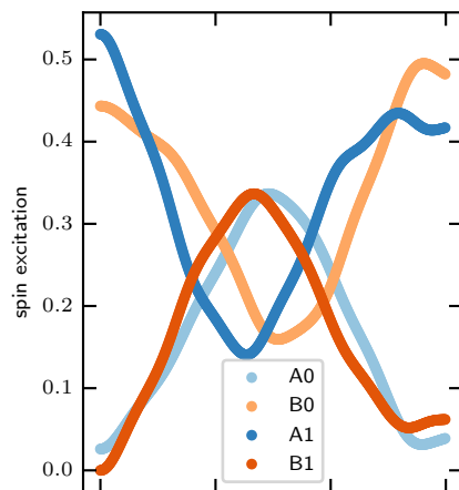
excited phonons: 5
