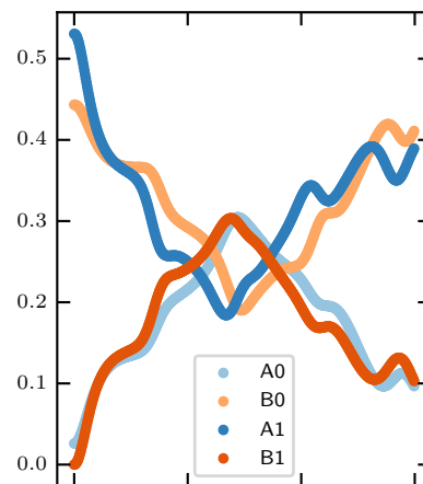
excited phonons: 15
