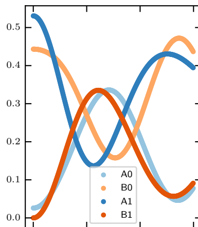
excited phonons: 10
