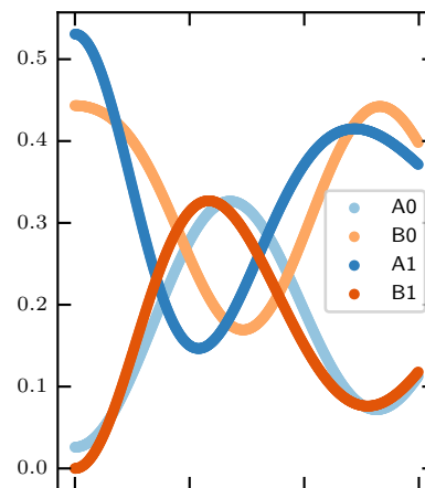
excited phonons: 15
